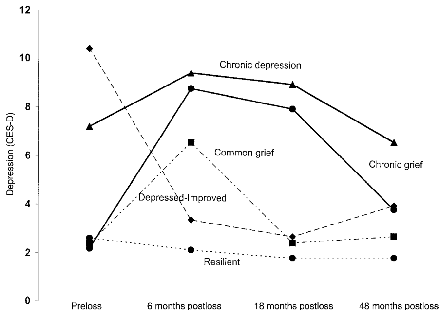
Figure 1. Patterns of depression from preloss to 48 months postloss ( N = 92 ).
