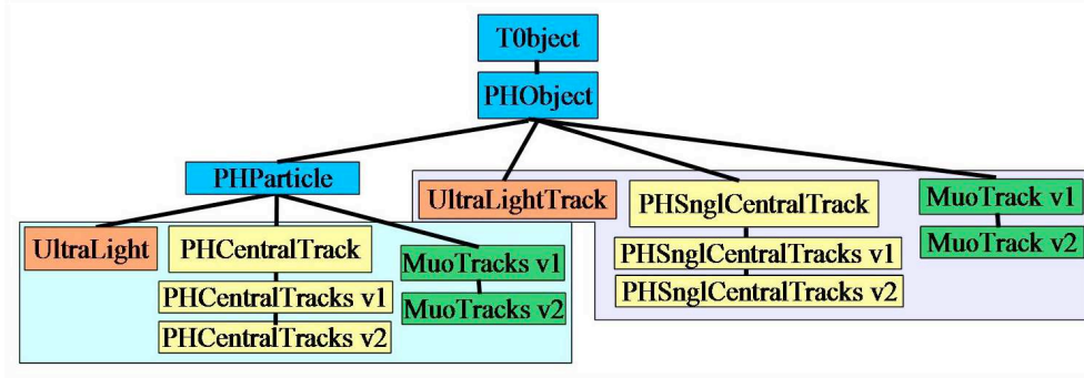
Figure 5.3: Diagram of the PHENIX data class inheritance tree.
