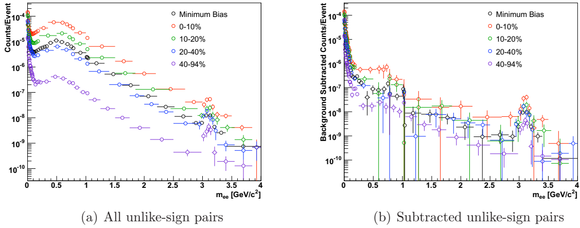
Figure 5.15: The minimum bias unlike-sign mass distributions displayed with the various centrality groupings. Both the background subtracted and unsubtracted spectra are shown.
