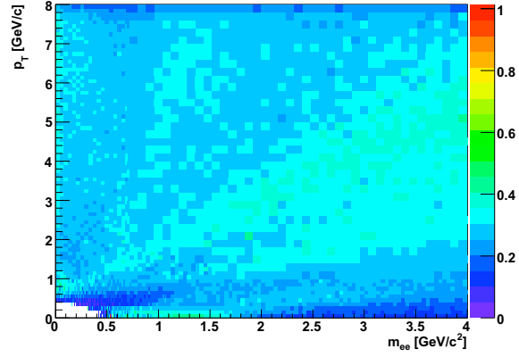
Figure 6.10: The efficiency as a function of mass and p_T .
