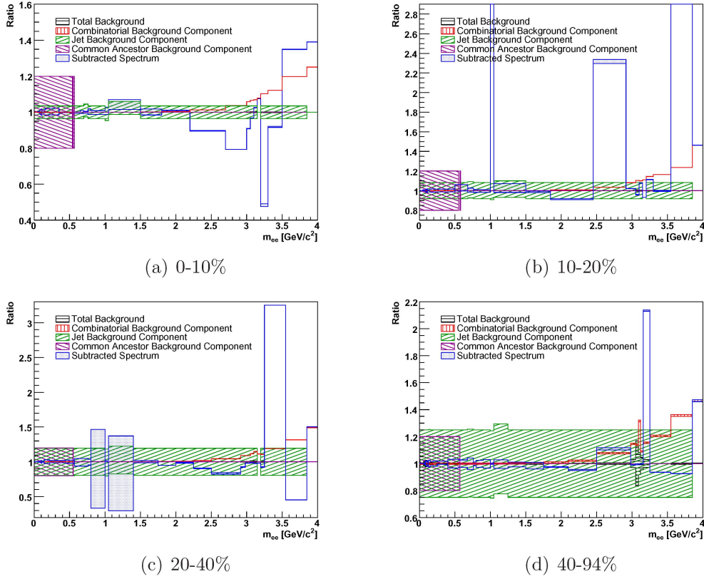
Figure 7.5: The ratio of the backgrounds and subtraction with the common ancestor component changed by 20% in each direction over the backgrounds and subtraction with the expected common ancestor component. The total background is shown in black with horizontal lines, the combinatorial background is red with vertical lines, the jet and common ancestor backgrounds are green and purple respectively with diagonal lines and the subtracted spectra are the blue dotted regions.
