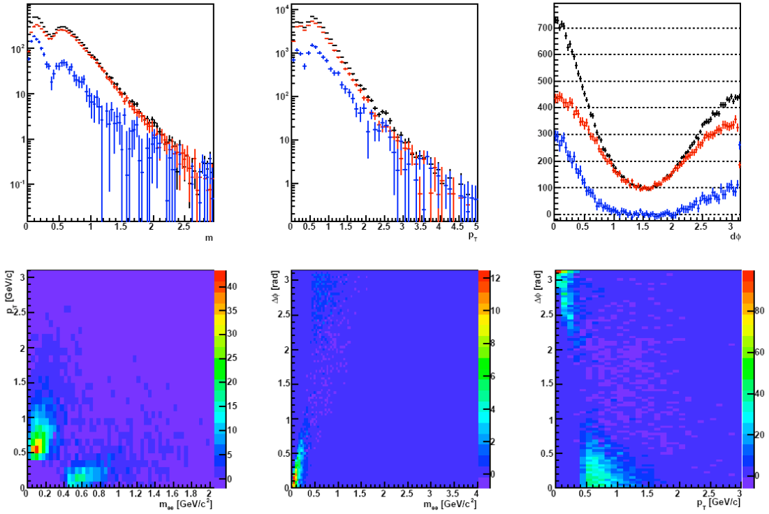
Figure 4.11: The top row shows the like-sign correlated jet pair mass, p_T , and \Delta\phi spectrum for all pairs (black), background event pairs (red) and background event subtracted pairs (blue). The second row shows the subtracted spectrum in different two-dimensional projections of mass vs. p_T , mass vs. \Delta\phi , and p_T vs. \Delta\phi .
