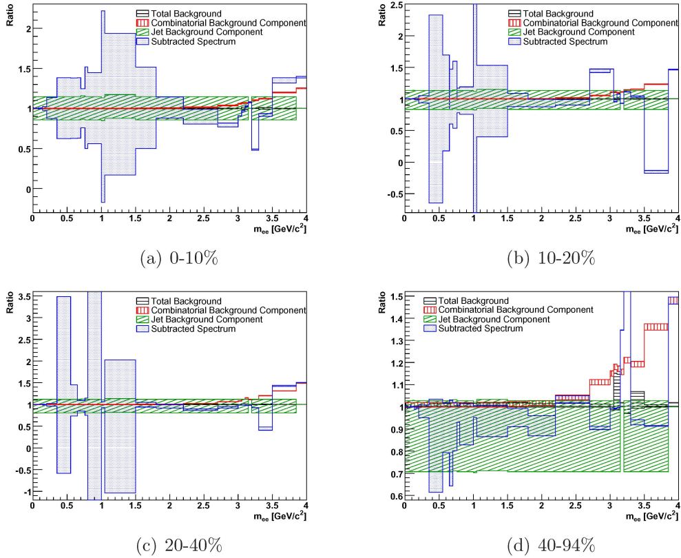
Figure 7.7: The ratio of the backgrounds and subtraction with the jet component shape altered to include the full away-side jet component and no away-side jet component over the backgrounds and subtraction with the expected jet component shape. The total background is shown in black with horizontal lines, the combinatorial background is red with vertical lines, the jet background is green with diagonal lines and the subtracted spectra are the blue dotted regions. The common ancestor background is unaffected by the away-side jet shape.
