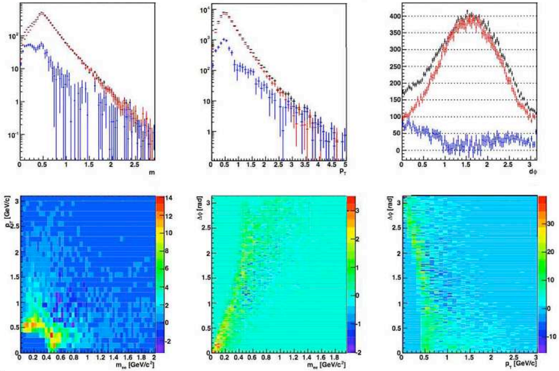
Figure 4.10: The top row shows the unlike-sign correlated jet pair mass, p_T , and \Delta\phi spectrum for all pairs (black), background event pairs (red) and background event subtracted pairs (blue). The second row shows the subtracted spectrum in two-dimensional projections of mass vs. p_T , mass vs. \Delta\phi , and p_T vs. d\phi .
