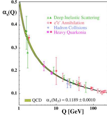
Figure 1.2: The coupling constant, \alpha_s , dependence on the momentum transfer, Q . Various experimental results are shown. The lines correspond to a pQCD calculation. [6]
