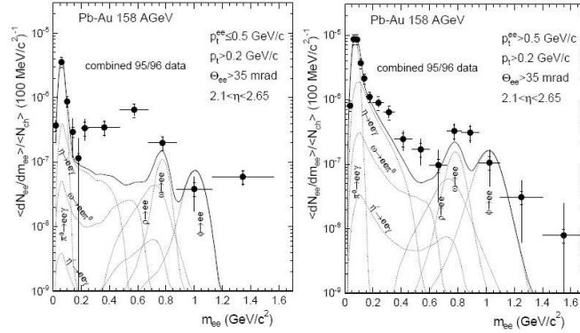
Figure 9.7: The CERES 158 AGeV Pb+Au spectra divided by p_T above and below 0.5 GeV/c. [59]
