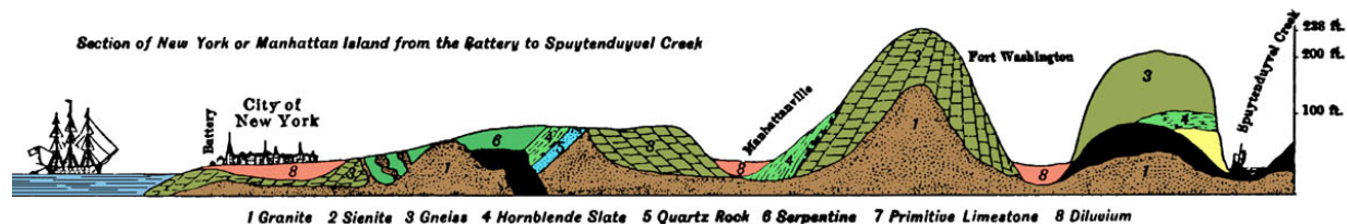
Figure 4 – S to N profile of Manhattan, from Battery (L) to Spuyten Duyvel Creek (R), showing shape of land surface (shaded, below) and inferred geological relationships as determined by Issachar Cozzens. (Adapted from G. P. Merrill, 1924, fig. 43, p. 238; after Cozzens, 1843).
