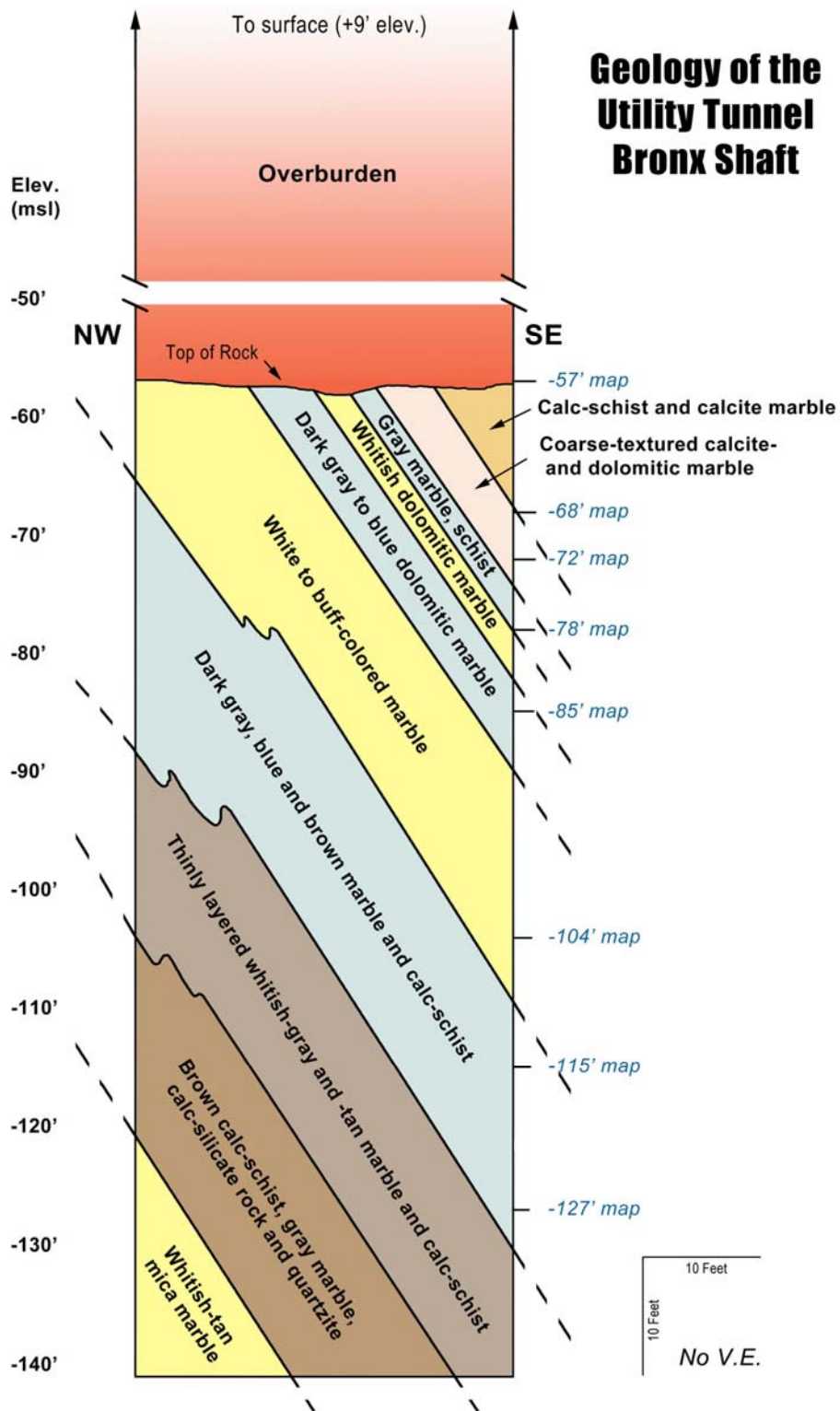
Figure 12 – NW-SE profile section across the Bronx shaft of the utility tunnel showing the homoclinal stratigraphy and the positions of the eight plan view maps (in blue) used to construct the section. (Geological mapping by C.M. and J.M. Merguerian, 2009.)
