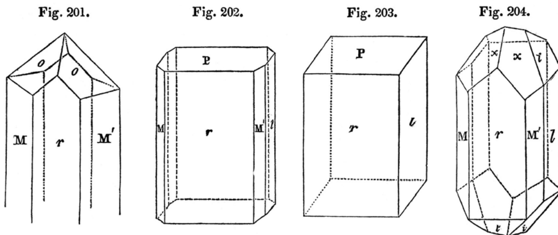
Figure 2 – Various crystal habits of white pyroxene (diopside) found by mineralogists in the Kingsbridge area, NYC as described on p. 291 in Beck (1842). Reproduced figures are found compiled on p. 487.)
