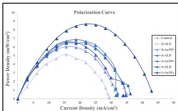
Figure 1: Graph of polarization curves (Power density vs current density) of the control electrodes, as well as 1, 3, and 5 cycles of Titanium Dioxide, with and without gold
