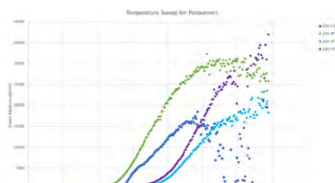
Figure 3: Temperature Sweep for poloxamer gels
