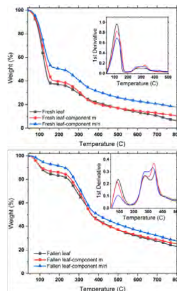
Figure 2 TGA results
