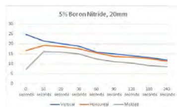
Figure 1) Temperature Difference for 5% B-N
