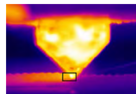
Fig. 1. Thermal imagery of lattices during printing process
