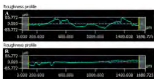
Figure 1: Roughness profiles of the Makerbot PLA samples (A) and the Ultimaker 2+ PLA samples (B)
