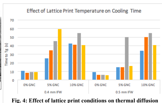
Fig. 4: Effect of lattice print conditions on thermal diffusion
