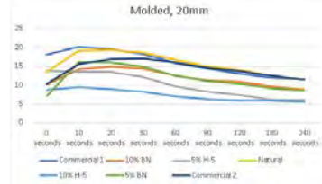
Figure 3) Temperature Difference for Molded Samples
