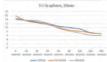
Figure 2) Temperature Difference for 5% Graphene
