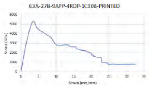
Figure 3: Stress Vs. Strain graph for Printed Flame Retardant Sample
