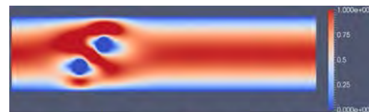
Figure 2: Simulation of multiple graphene particles in PLA filament
